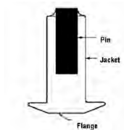
Figure 1: A typical stud.
