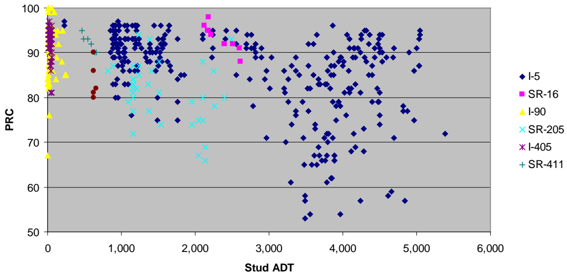
Figure 10: Distribution of PRC vs. stud ADT by western highway.
